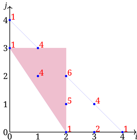
Figure 11: Critical triangle of the weighted Newton polygon \Delta_{29} . Notice that per our definition, the lines i = 2 and j = 3 themselves are not considered as part of the critical triangle.
