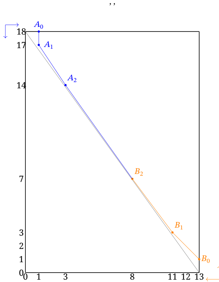
Figure 14: Markov sail for Example 8.5.
