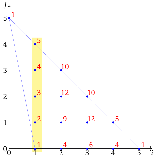
Figure 9: Weighted Newton polygon of M_{1/5} with the highlighted coefficients on the line i = 1 .
