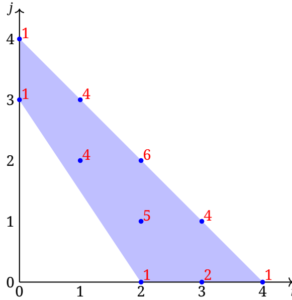
Figure 7: ‘Weighted’ Newton polygon of the Markov polynomial M_{2/3} .
