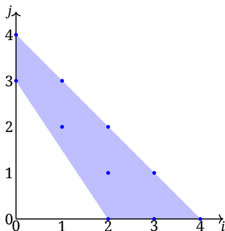
Figure 6: Newton polygon \Delta_\rho , of the Markov polynomial M_\rho, \rho = \frac{2}{3} .
