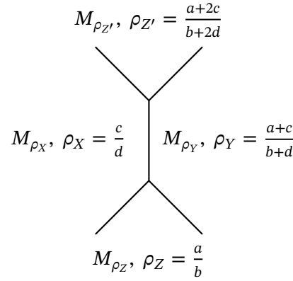
Figure 5: Section of the Conway topograph showing correspondence.
