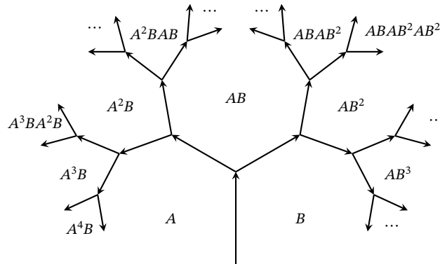
Figure 15: The Cohn tree.
