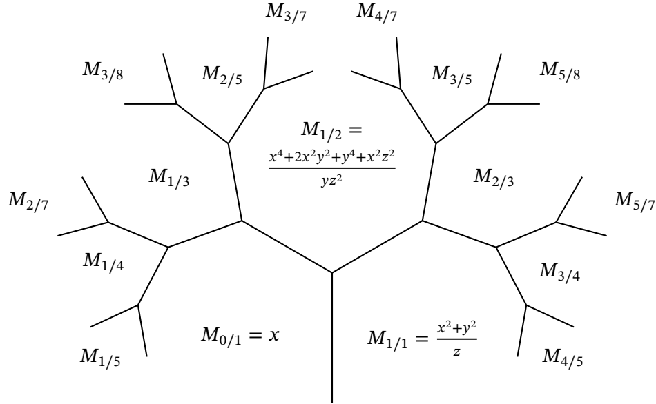
Figure 3: Markov polynomials on the Conway topograph.
