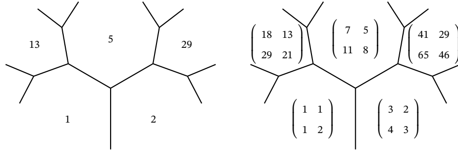
Figure 16: Cohn and Markov trees related by trace map
