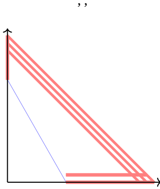
Figure 8: Lines on the Newton polygon where the coefficients are explicitly known.
