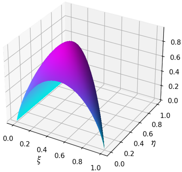
Figure 10: Graph of the entropy for Fibonacci polynomials.
