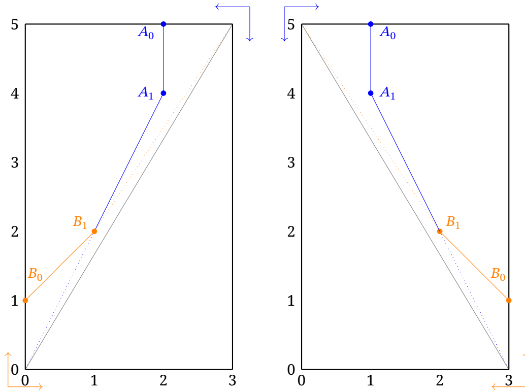
Figure 13: (Left) Combined sail for the rational \frac{5}{3} ; (Right) the reflection in the line x = a/2 .
