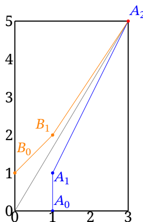
Figure 12: Klein Diagram for the rational \frac{5}{3}
