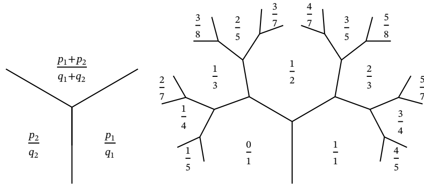
Figure 1: Rationals in [0, 1] represented on the Conway topograph.
