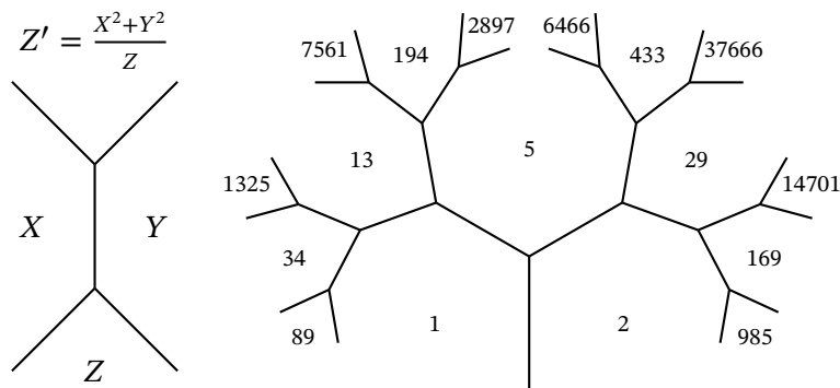
Figure 2: Markov numbers represented on the Conway topograph.
