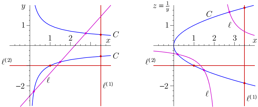
Fig. 3 The curve C in \mathbb{P}^1 \times \mathbb{P}^1 is defined by xy^2 = 1 and x = z^2 = (1/y)^2 in two distinct affine charts \mathbb{C} \times \mathbb{C} . Its witness collection is ((W_1, \ell^{(1)}), (W_2, \ell^{(2)})) , where W_i = C \cap \ell^{(i)}
