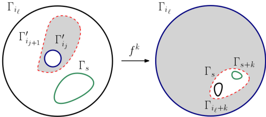
Fig. 1 On the left, the configuration of curves \Gamma'_{i_j}, \Gamma'_{i_{j+1}} and their f^k -images (namely, \Gamma_{i_\ell} and \Gamma_s resp.) are shown. Since \Gamma_s is contained in the annular domain A = A(\Gamma'_{i_{j+1}}, \Gamma'_{i_\ell}) , its image under f^k maps onto a curve \Gamma_{s+k} contained in A(\Gamma_{i_\ell+k}, \Gamma_s) . Colors match their image (color figure online)
