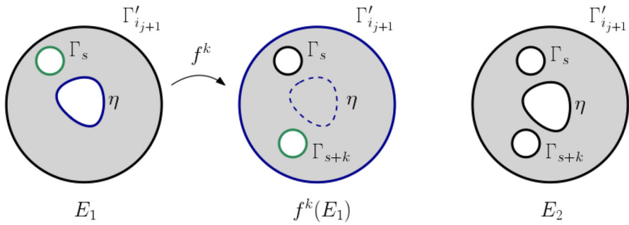
Fig. 2 The only remaining possible location of \Gamma_{s+k} with respect to the boundaries of E_1 is shown. E_1 is the grey region bounded by \Gamma'_{i_{j+1}}, \eta and \Gamma_s . Its conformal image, f^k(E_1) , is shown in grey and is bounded by \Gamma'_{i_{j+1}} = f^k(\eta) , \Gamma_s = f^k(\Gamma'_{i_{j+1}}) and \Gamma_{s+k} = f^k(\Gamma_s) (colors match their image). The 4-connected region E_2 is obtained by removing the topological disk \overline{D_{s+k}} from E_1 (color figure online)
